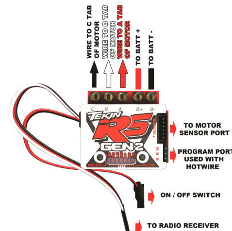
MOTOR TYPE (MT) SETTINGS MT1 / LED 1 - FWD/BRK MT2 / LED 2 - FWD/REV IMMEDIATE MT3 / LED 3 - FWD/BRK/REV DELAY
