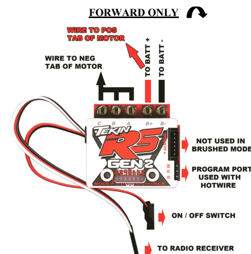
MOTOR TYPE (MT) SETTINGS MT4 / LED 4 - FWD/BRK
